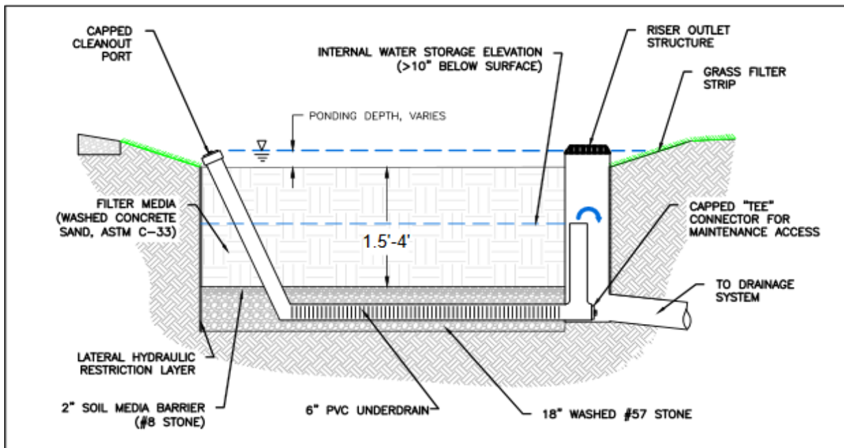
Figure B: Generic Media Filter BMP Detail - County of San Diego LID Handbook
