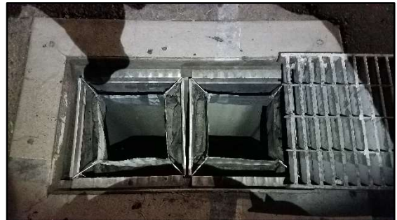
Figure 4. Installed FloGard® GIB – parallel systems.
