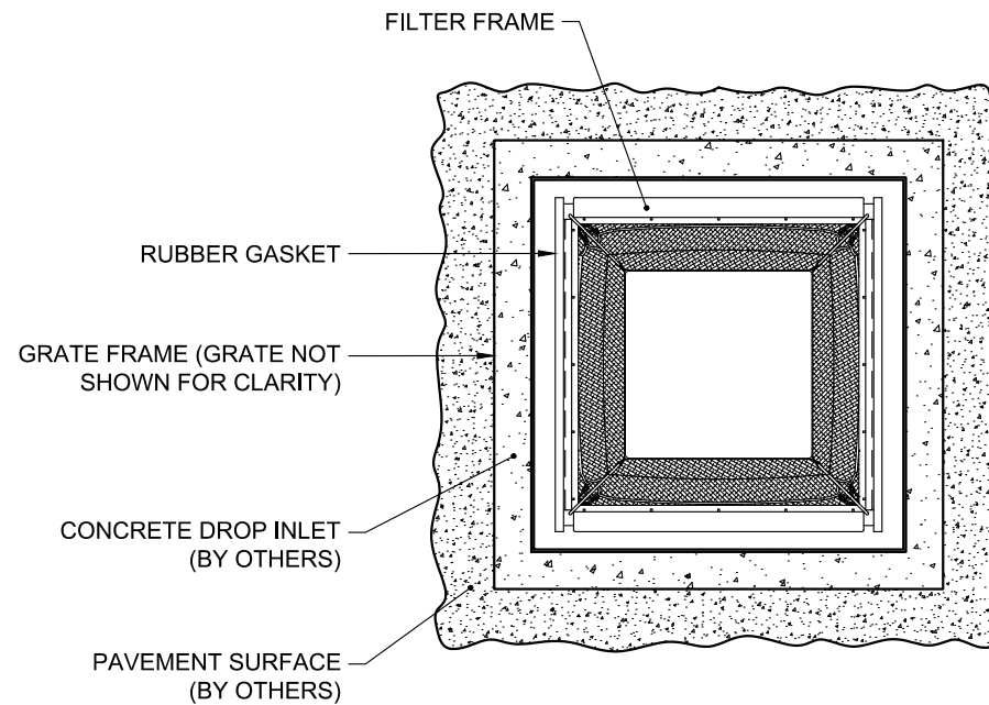
PLAN VIEW (GRATE NOT SHOWN FOR CLARITY)
