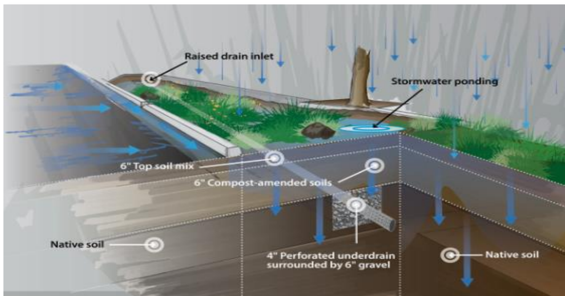
Figure B: Generic Urban Infiltration Trench Detail
