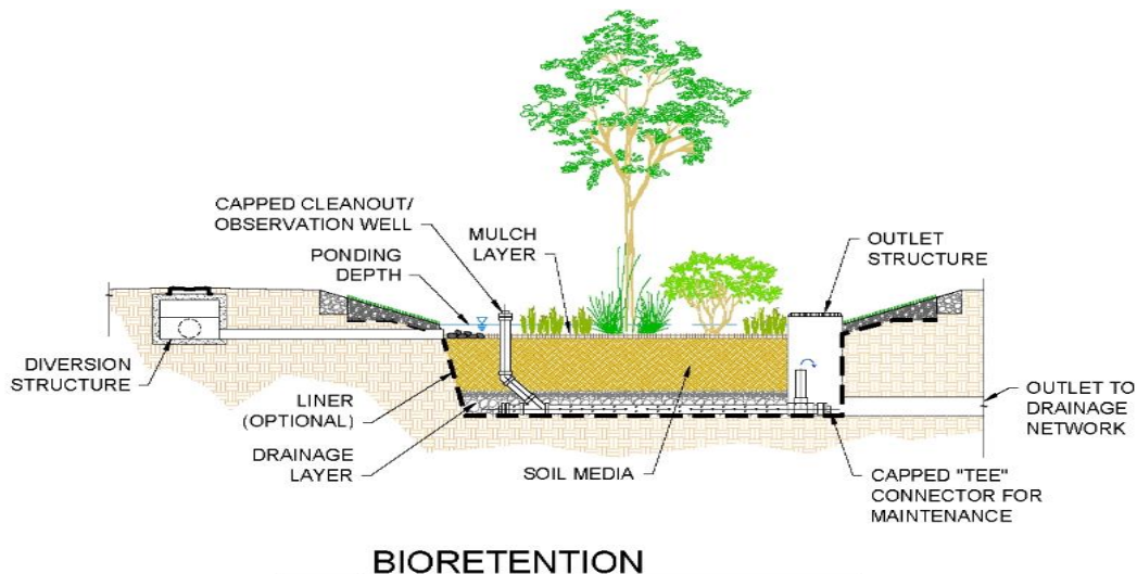
Figure B: Schematic Diagram of a Generic Bioretention System
