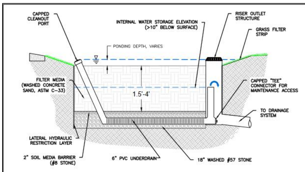
Figure B: Schematic Detail of a Generic Media Filter
